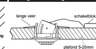
Fig. 4: montage sensor
