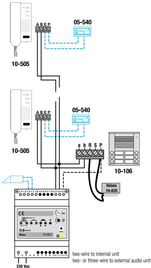
Fig. 4: complete wiring diagram
